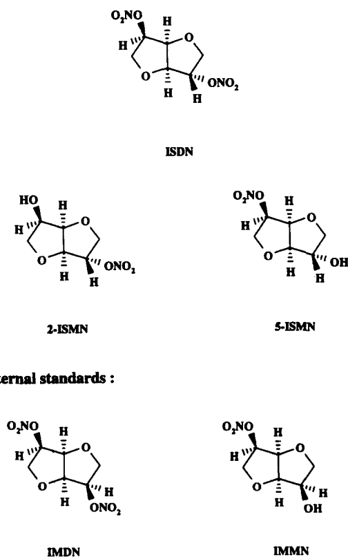
Fig. 1. Chemical structures of ISDN, mononitrate metabolites and internal standards.
