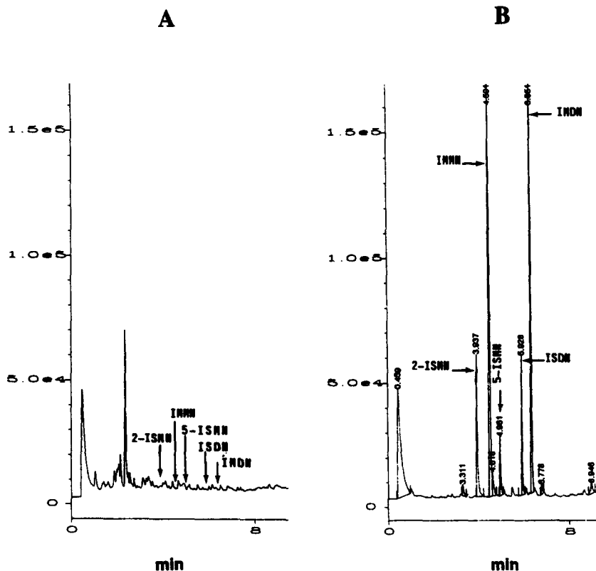
Fig. 2. Examples of chromatograms: (A) extract of 1 ml drug-free plasma; (B) plasma samples spiked with 14.6 ng of ISDN, 18.5 ng of 2-ISMN, 12.2 ng 5-ISMN, 56.6 ng IMDN and 84 ng IMM.
